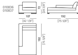
Chaise-longue with right or left short arm
